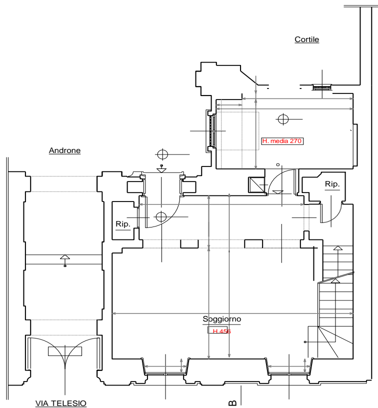
PIANO TERRA SCALA 1:100
